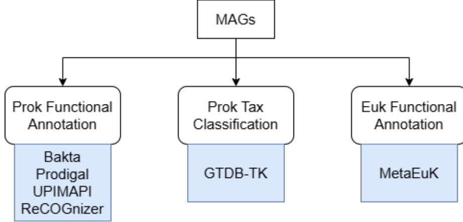
Fig. 1. Architectural overview of the metagenomic pipeline. MAGs are routed according to their domain: prokaryotic bins undergo taxonomic and functional annotation (GTDB-Tk, Prodigal, Bakta, UPIMAPI, and reCOGnizer), while eukaryotic bins are processed via MetaEuk, with all data converging into a centralized Integrated Annotation Table.
